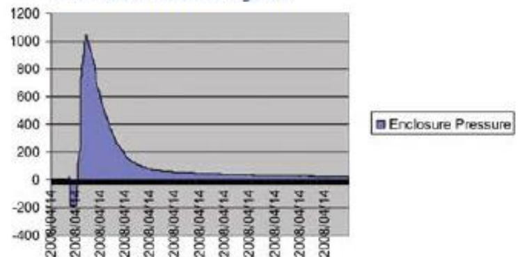
FM200 Sealed Room Discharge Test
